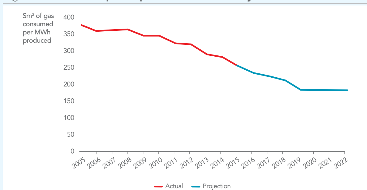
Figure 10 Gas Required per Unit of Electricity Generation – MIS
