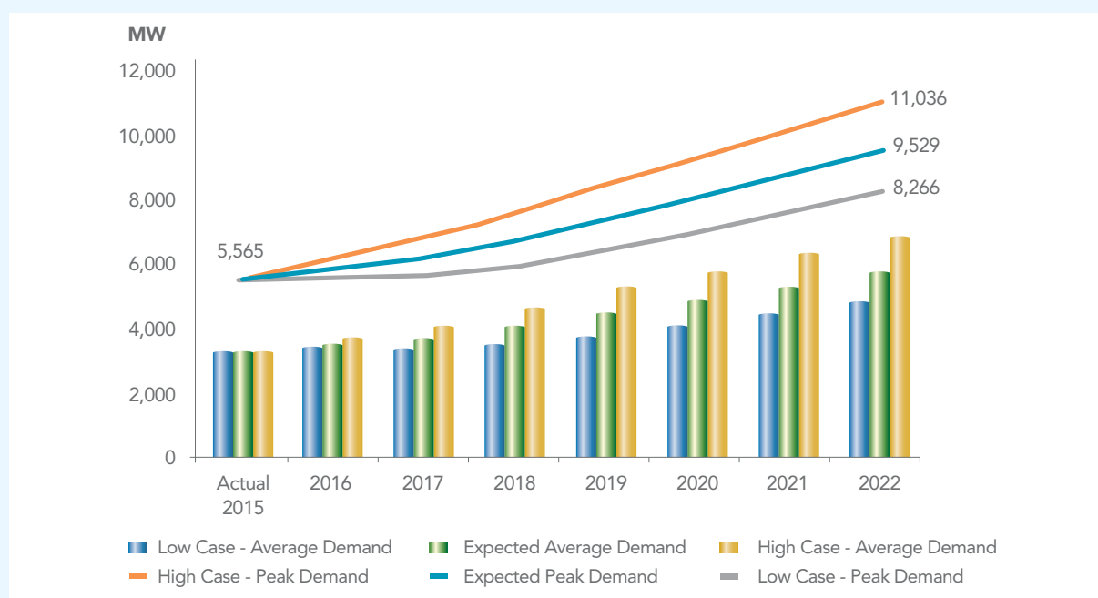
Figure 1 Electricity Demand Projections–MIS
