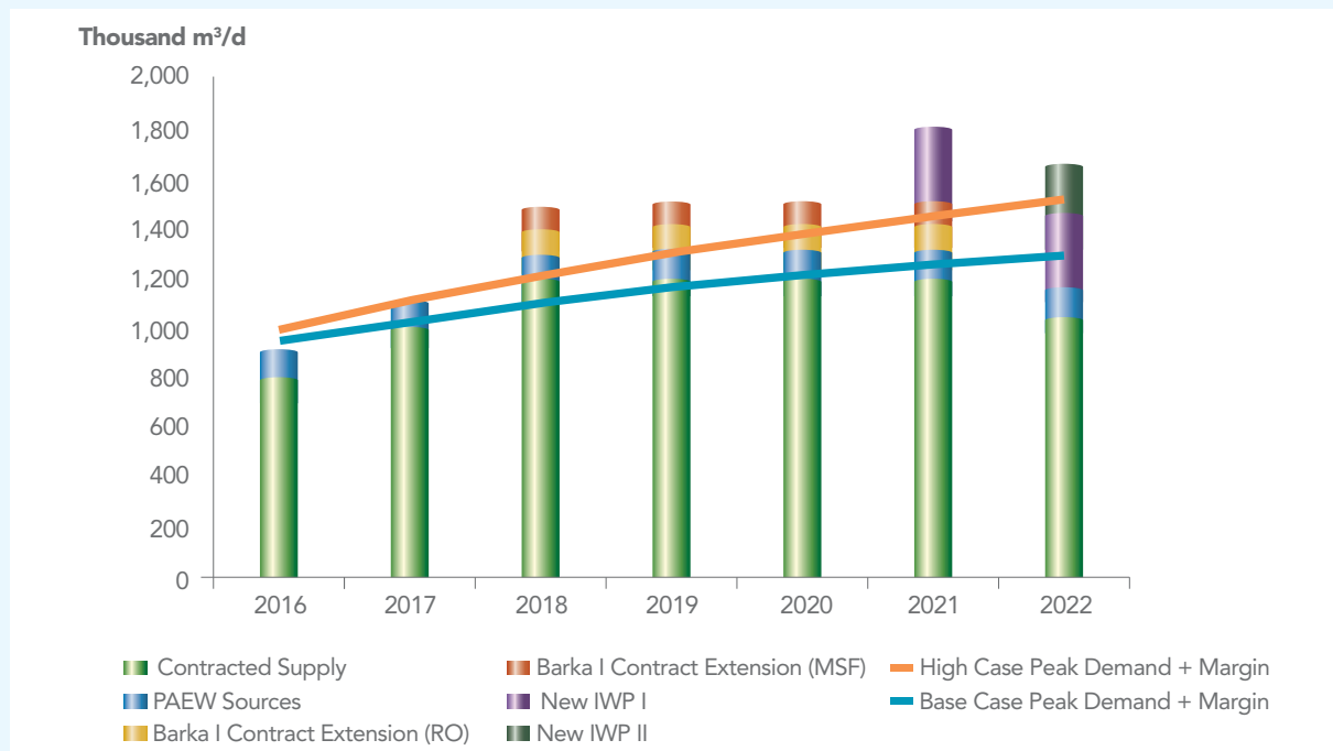
Figure 6 Desalinated Water Capacity Requirements – Interconnected Zone
