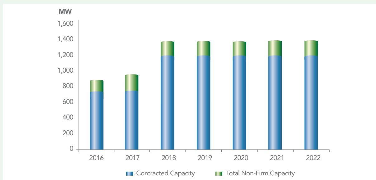
Figure 12 Total Power Generation Resources – Dhofar Power System
