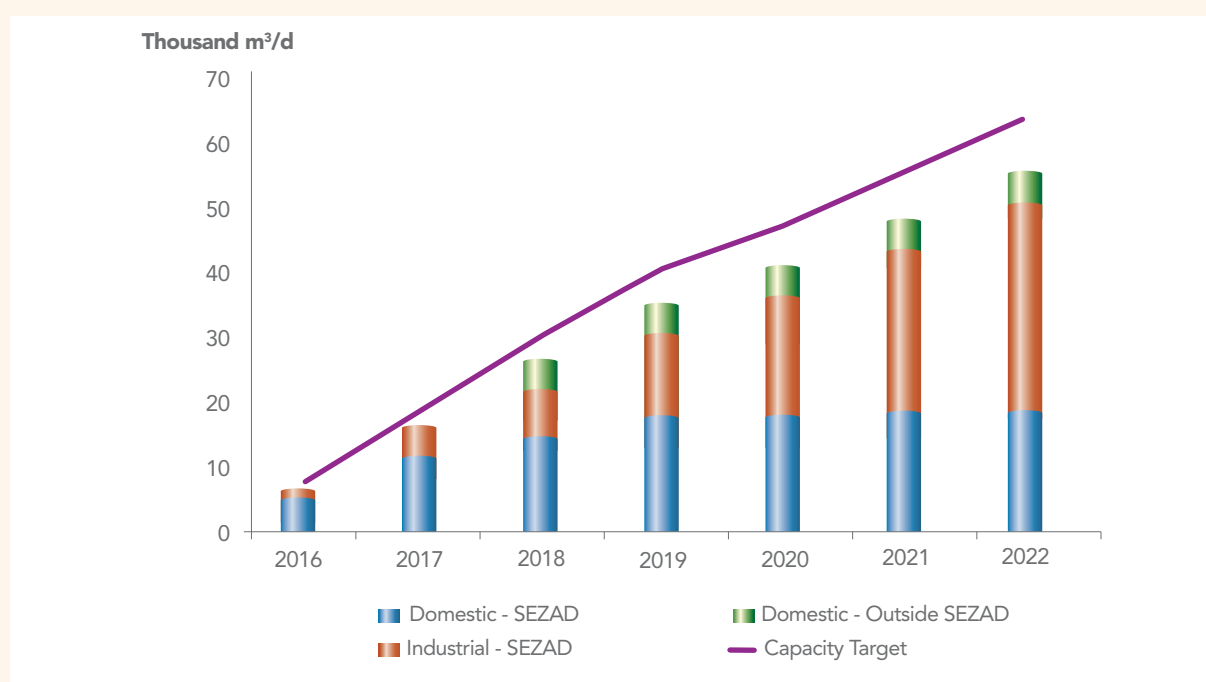
Figure 21 Peak Water Demand and Capacity Requirement - Ad Duqm Zone
