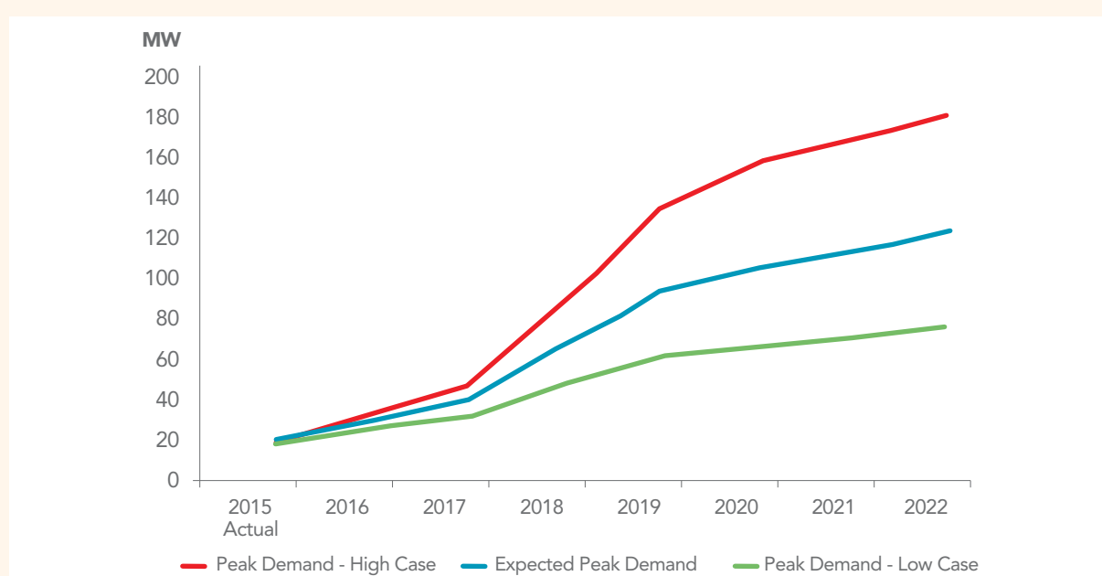
Figure 17 Electricity Demand Projections – Ad Duqm
