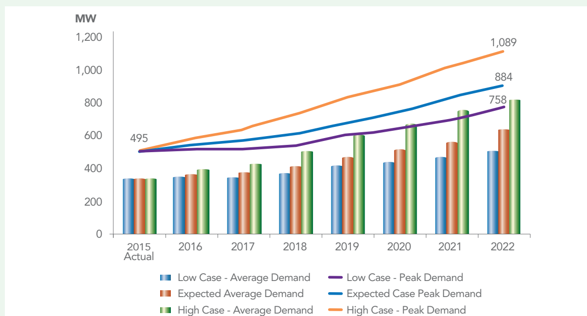
Figure 11 Electricity Demand Projections – Dhofar Power System
