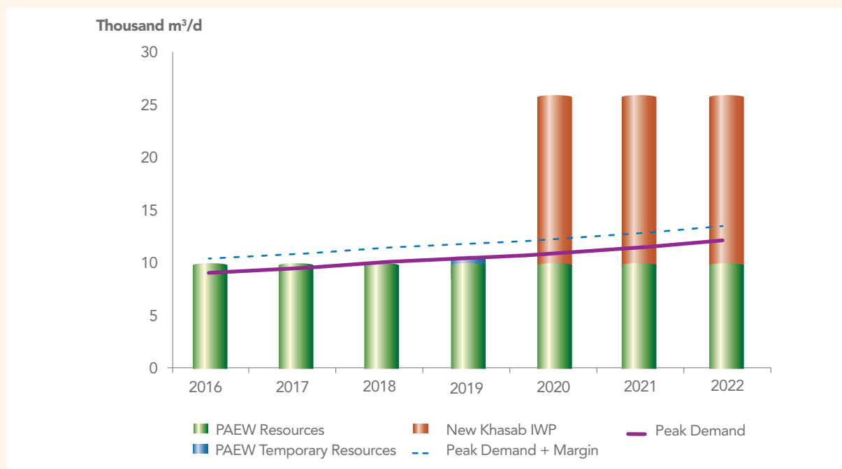
Figure 24 Water Supply and Demand Balance – Musandam
