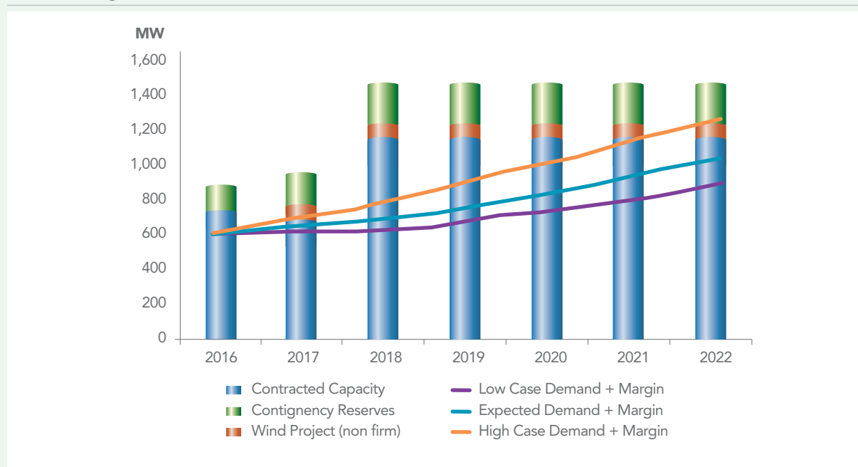
Figure 13 Future Power Generation Capacity Requirements – Dhofar Power System
