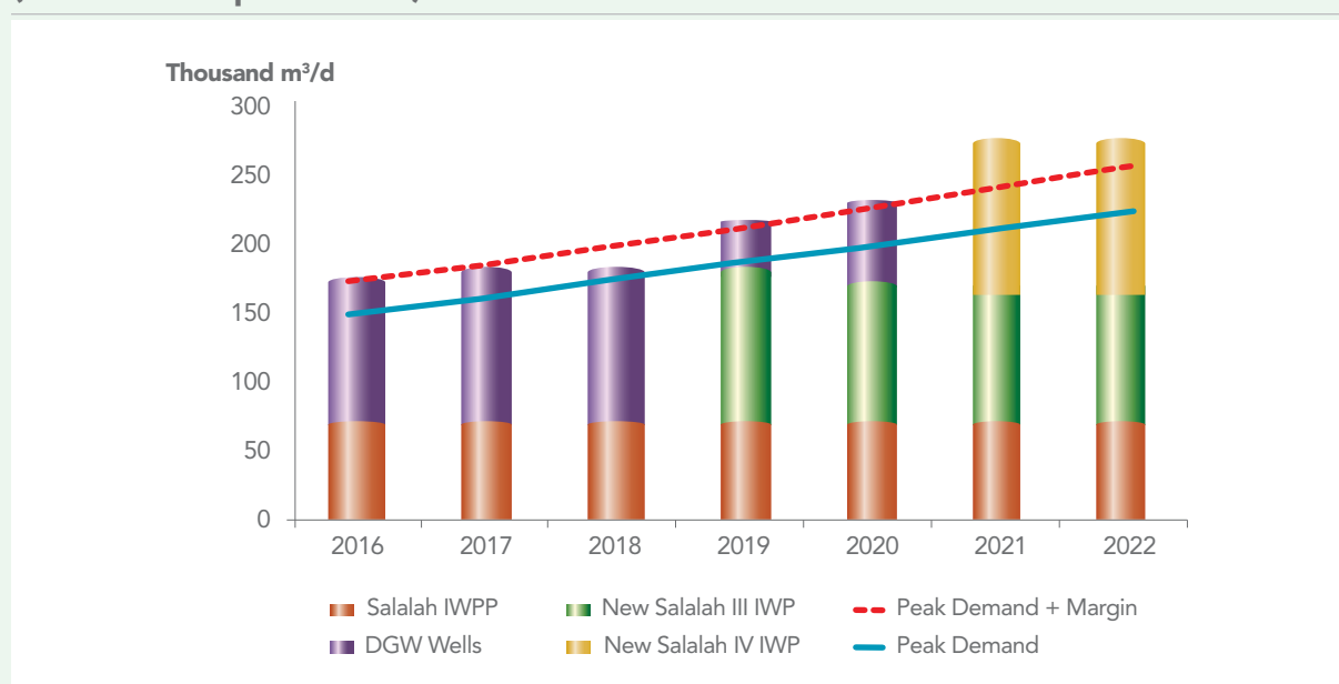
Figure 15 Future Desalinated Water Capacity Requirement – Dhofar (Salalah/Taqqa/Mirbat)
