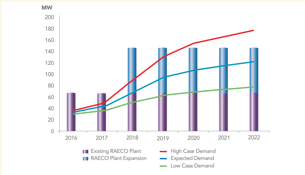
Figure 19 Future Power Generation Expansion Plan – Ad Duqm
